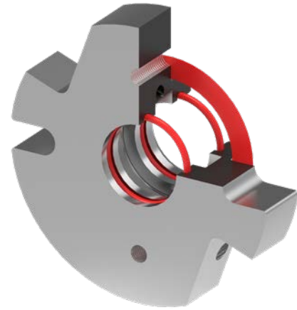
O-Pro® Cartridge Seal Cutaway
